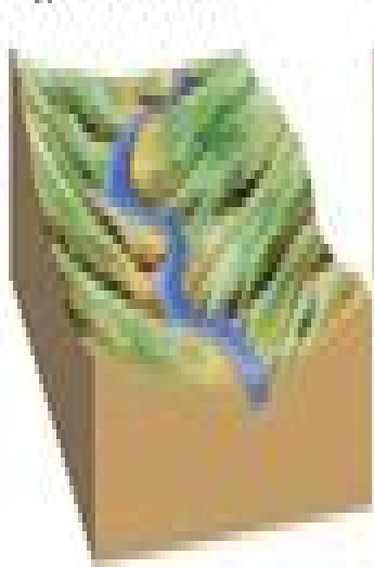
river carving a valley
