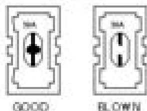
MAX-FUSE CARTRIDGE TOP VIEW
