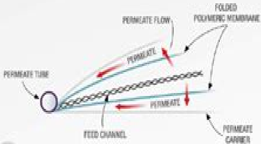
3 Cross section of a membrane leaf
