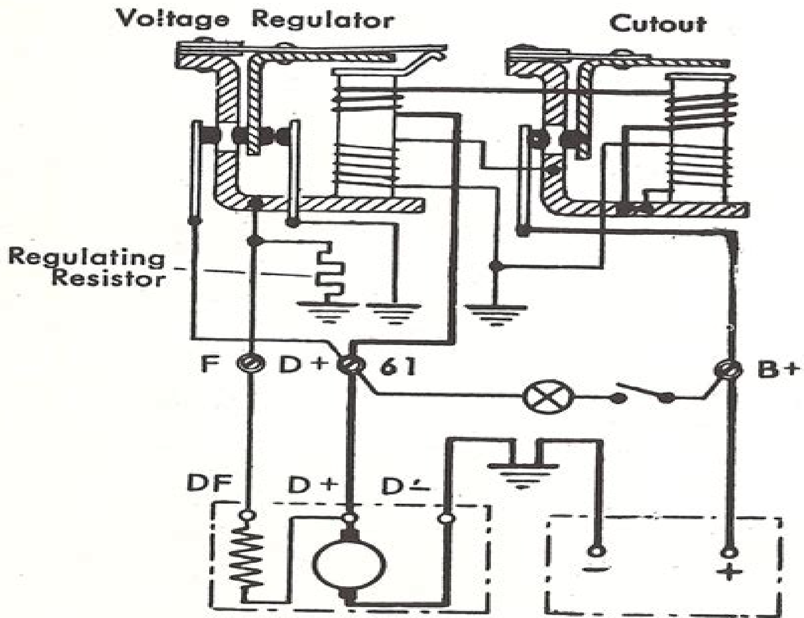
Wiring diagram of the regulator.
